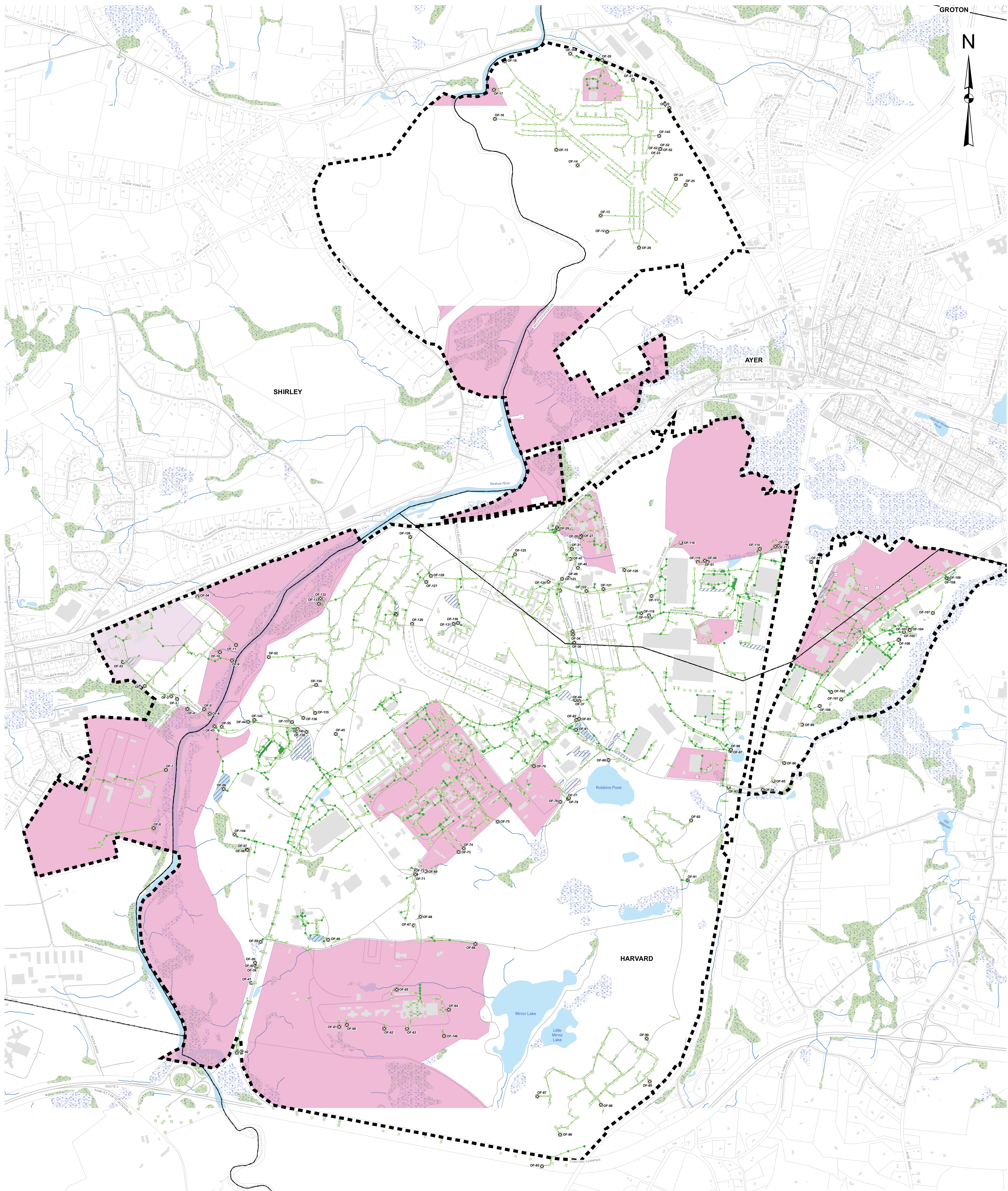
FIGURE 1 MASSACHUSETTS DEVELOPMENT FINANCE AGENCY MS4 COMPLIANCE DEVENS DRAINAGE SYSTEM MAP MARCH 2018 SCALE: NOTED
